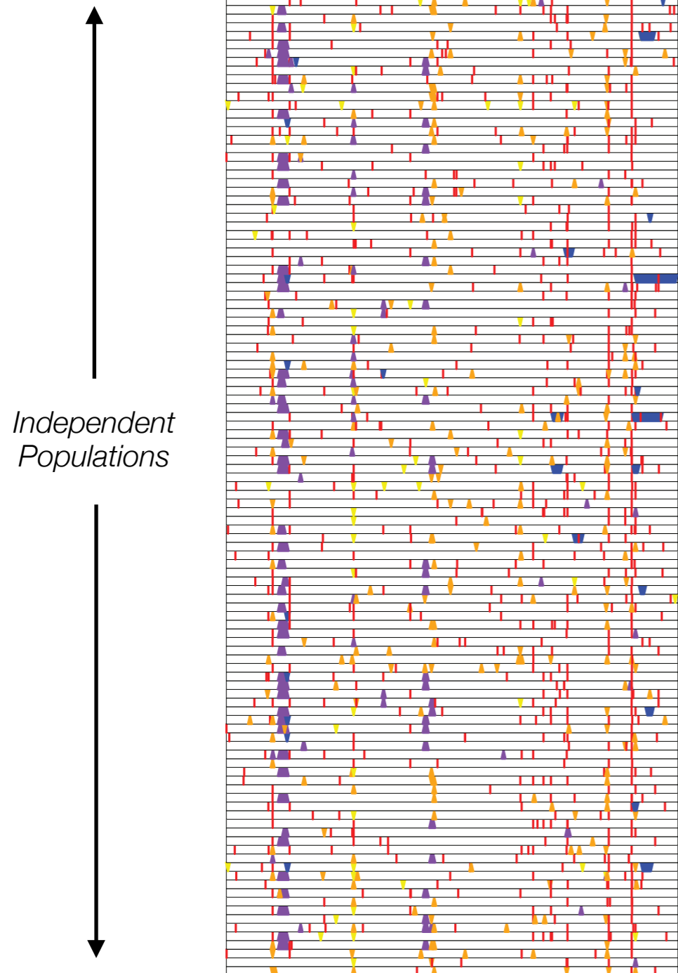
Mutations observed in genome
